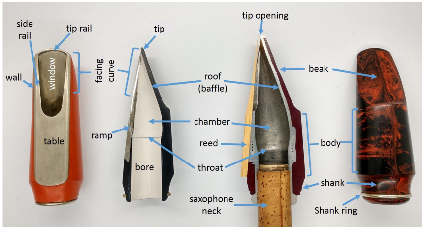
FIGURE 1. The parts of a saxophone mouthpiece. From left, a hard-rubber Holton alto saxophone with a nickel-silver core and table; cross-section of a hard-rubber Naujoks-McLaughlin Sil-Va-Lae alto (nickel-silver table painted white on the interior for photography); cross section of a Bakelite-and-metal Holton Perfected model c-melody attached to a saxophone neck; an unbranded marbled hard-rubber alto. Author's photo.
