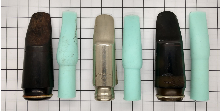
FIGURE 2. Wood, metal, and hard-rubber mouthpieces paired with silicone-rubber casts of each interior cavity. From left, an unbranded wood alto; Goldbeck Superb nickel-silver alto; Conn eagle trademark hard-rubber alto. The casts show the exact shape of the respective large chambers. Gridlines in the background of this and subsequent images are one centimeter apart. Author's photo.
