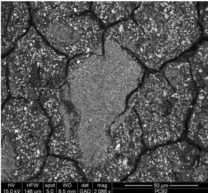
FIGURE 15. Backscattered electron image of a bright orange Holton hard-rubber body alto saxophone mouthpiece. A 50 micron-wide grain of finer material is seen in the center of the image. Brightest grains in the surrounding material are mercury sulfide (cinnabar). Darker gray and generally smaller grains are predominantly barium sulfate (barite). Cracks seen in black are partially filled with organic material; these result from aging of the hard rubber, not from being subjected to the low vacuum in the chamber of the microscope. Author's photo.
