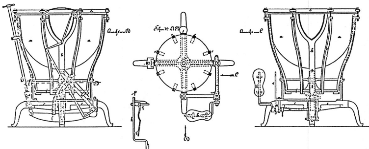
FIGURE II. Diagram of Pittrich's pedal tuning device. From patent specification no. 15199.
