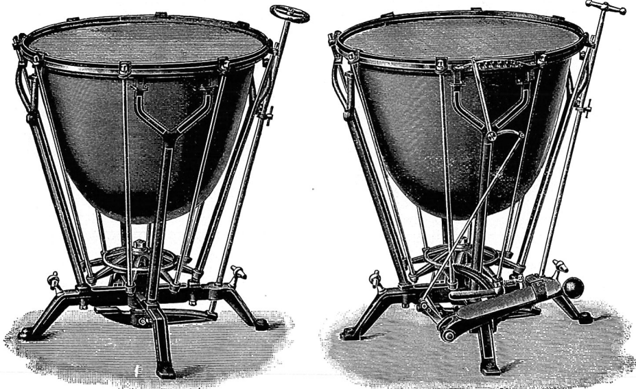
FIGURE 12. Pfundt/Hoffmann kettledrum (left) and a drum of the same type with a Pittrich pedal tuning device installed (right). From E. Teuchert and E. W. Haupt, Musikinstrumentenkunde in Wort und Bild .
