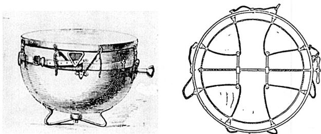
FIGURE 4. Cable-tuned machine drum invented by Cornelius Ward (1837). Side view from Ernst Pfundts Paukenschule ; top view from the Transactions of the Society of Arts, Manufactures and Commerce .
